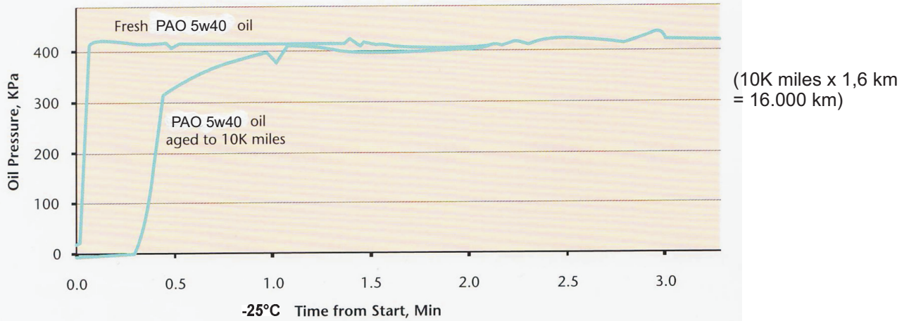
FIGURE 5 Oil Pressure Build-Up Using PAO base fluid
